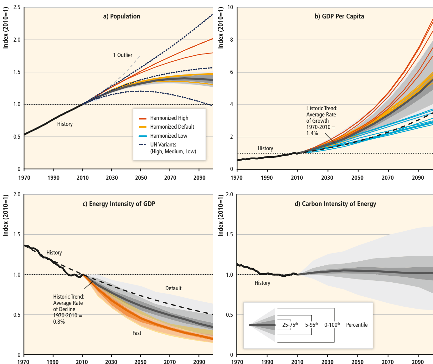
Figure 6.1 | Global baseline projection ranges for Kaya factors. Scenarios harmonized with respect to a particular factor are depicted with individual lines. Other scenarios are depicted as a range with median emboldened; shading reflects interquartile range (darkest), 5th—95th percentile range (lighter), and full range (lightest), excluding one indicated outlier in panel a) Scenarios are filtered by model and study for each indicator to include only unique projections. Model projections and historic data are normalized to 1 in 2010. Gross domestic product (GDP) is aggregated using base-year market exchange rates. Energy and carbon intensity are measured with respect to total primary energy. Sources: UN (2012), WG III AR5 Scenario Database (Annex II.10). Historic data: JRC/PBL (2013), IEA (2012a), see Annex II.9; Heston et al. (2012), World Bank (2013), BP (2013).
